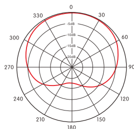
Polar Pattern
