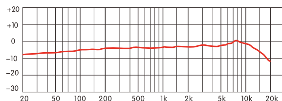
Frequency Response:
