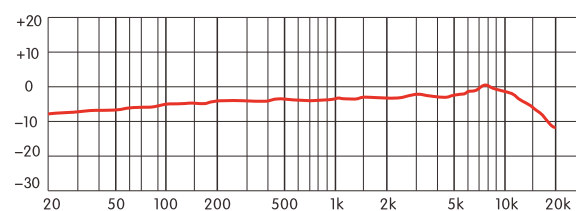
Frequency Response:
