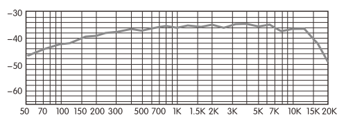
Frequency Response
