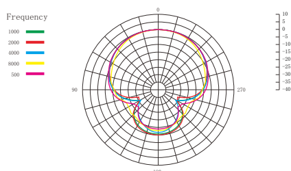
Polar Pattern
