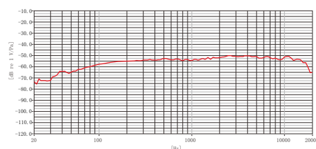
Frequency Response
