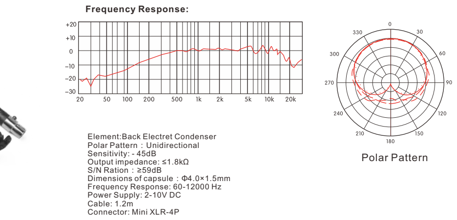
LM-C480 Unidirectional
