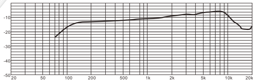
Frequency Response
