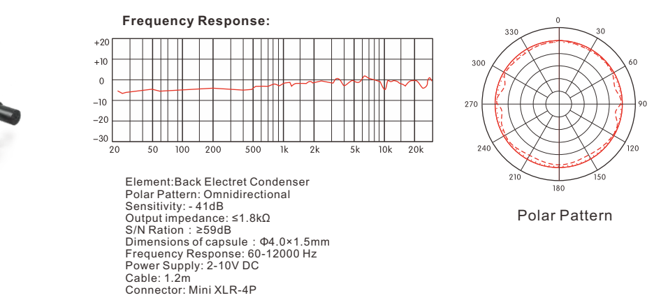
LM-C550 Omnidirectional
