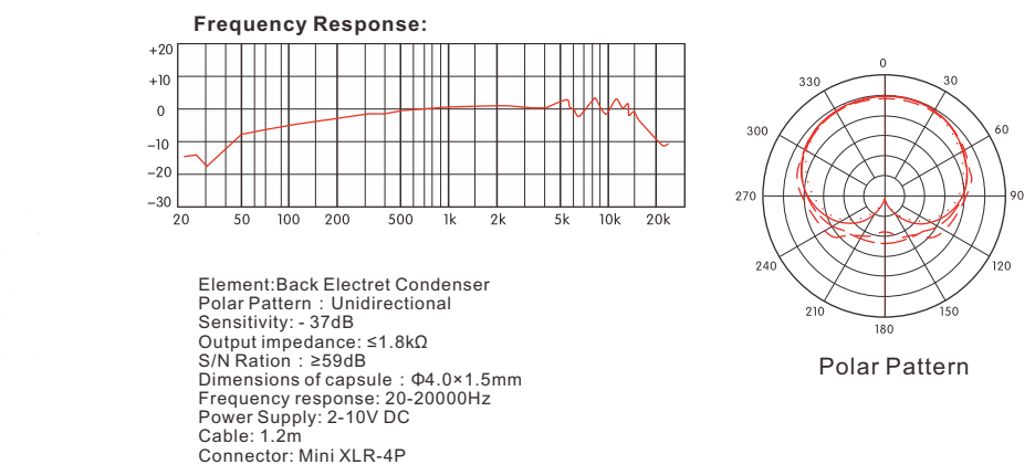
LM-C460 Unidirectional
