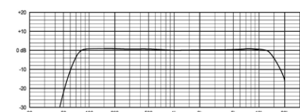
Frequency Response
