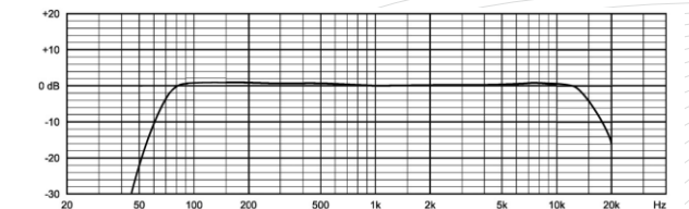
BM-112 Frequency Response 0dB=18 mV/Pa
