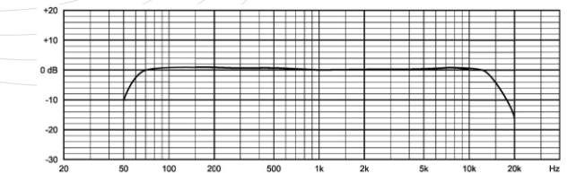
BM-113 Frequency Response 0dB=18 mV/Pa
