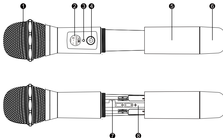
Handheld microphone (EH-6200)
